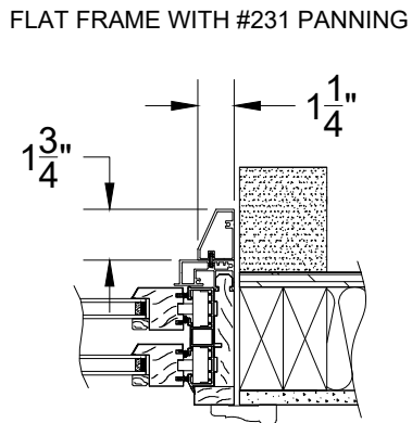
FLAT FRAME WITH #231 PANNING
