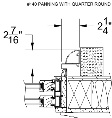
#140 PANNING WITH QUARTER ROUND
