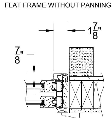
FLAT FRAME WITHOUT PANNING
