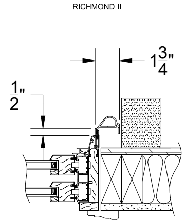
FLAT FRAME WITH QUARTER ROUND PANNING
